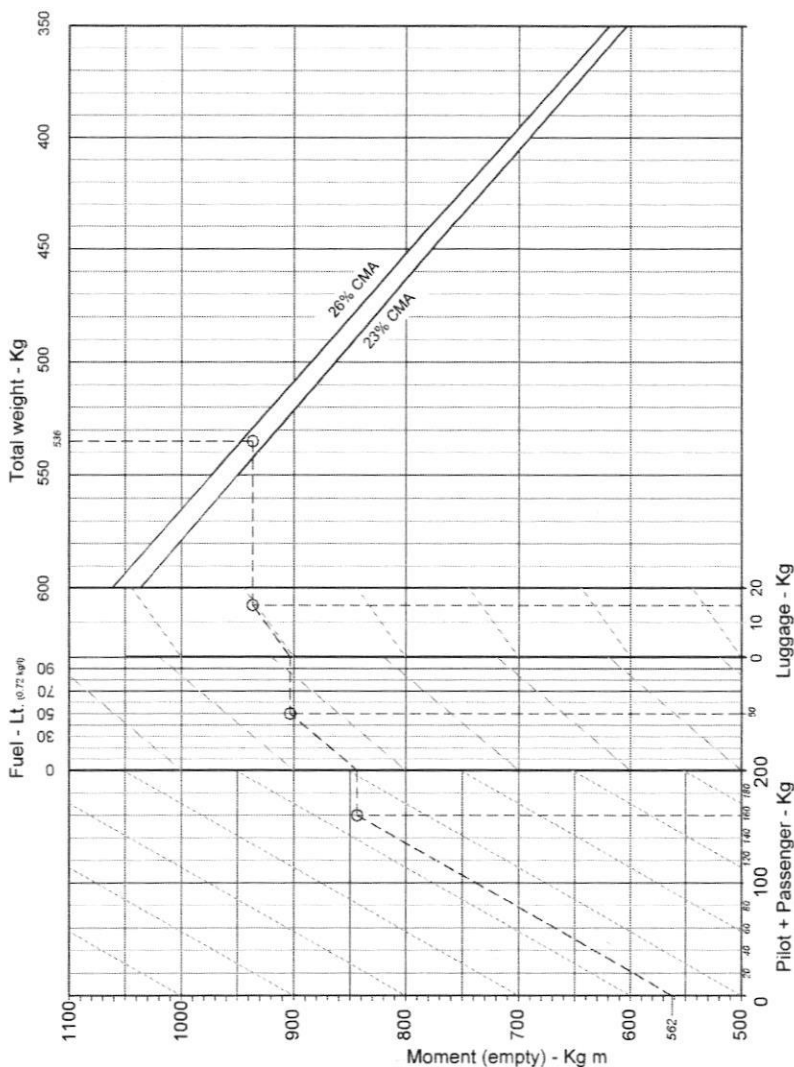
FIG. 6-1 Weight & balance chart
