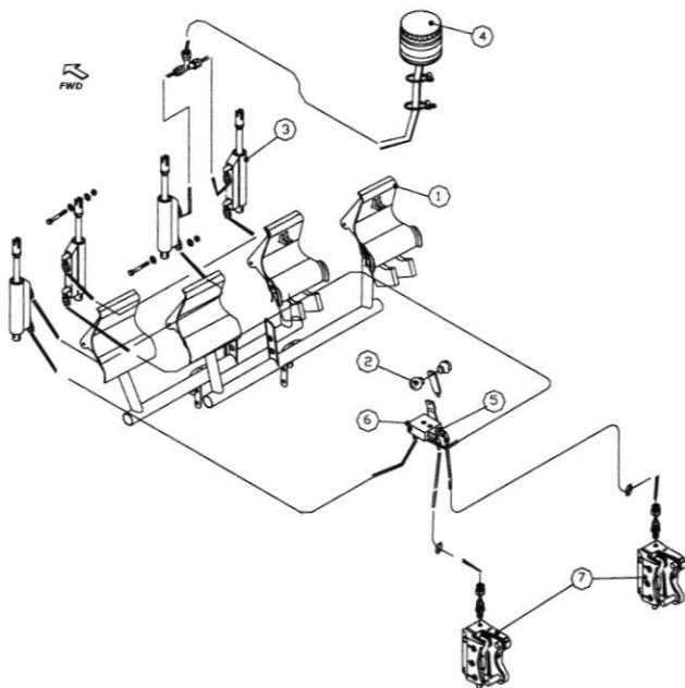
Figure 9-2 Differential brake system
