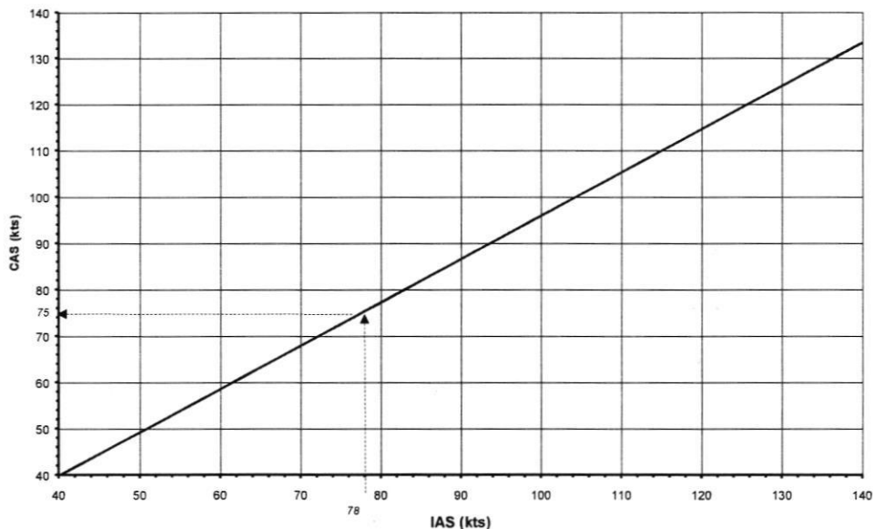
Fig. 5-1. CALIBRATED VS INDICATED AIRSPEED (BOTH MTOW)
