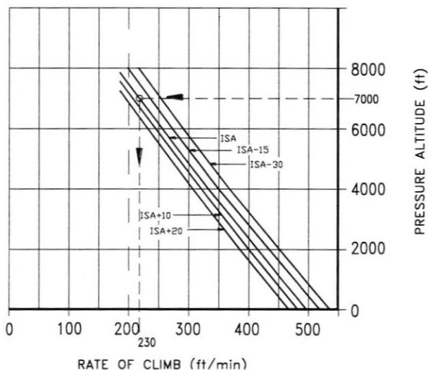
Fig.5-6. BALKED LANDING (MTOW=550KG)
