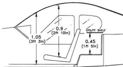
Fig 6-4. CABIN DIMENSIONS
