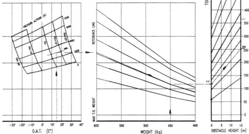
Fig. 5-4. TAKEOFF PERFORMANCE
