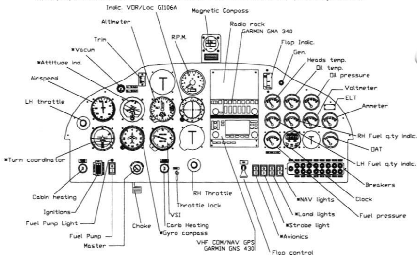
Fig. 7-2. INSTRUMENT PANEL
