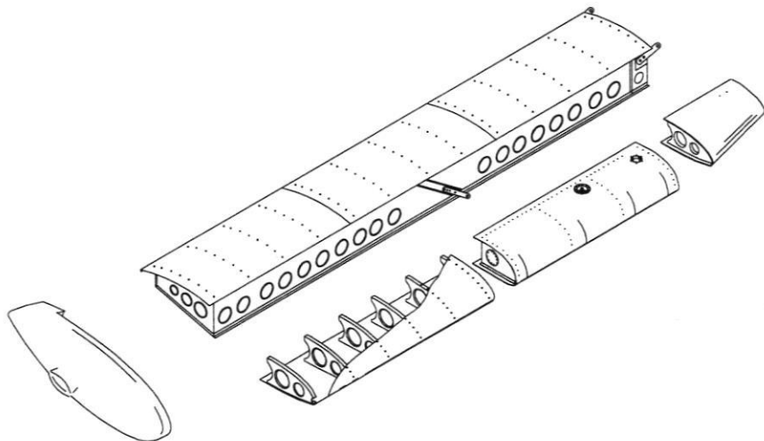
Fig. 7-1. RIGHT WING EXPLODED VIEW
