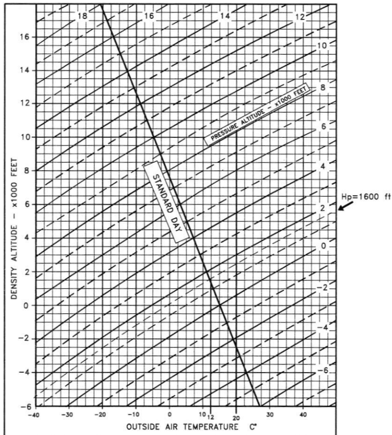
Fig. 5-2. ICAO CHART
