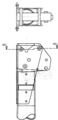
Hook connection
