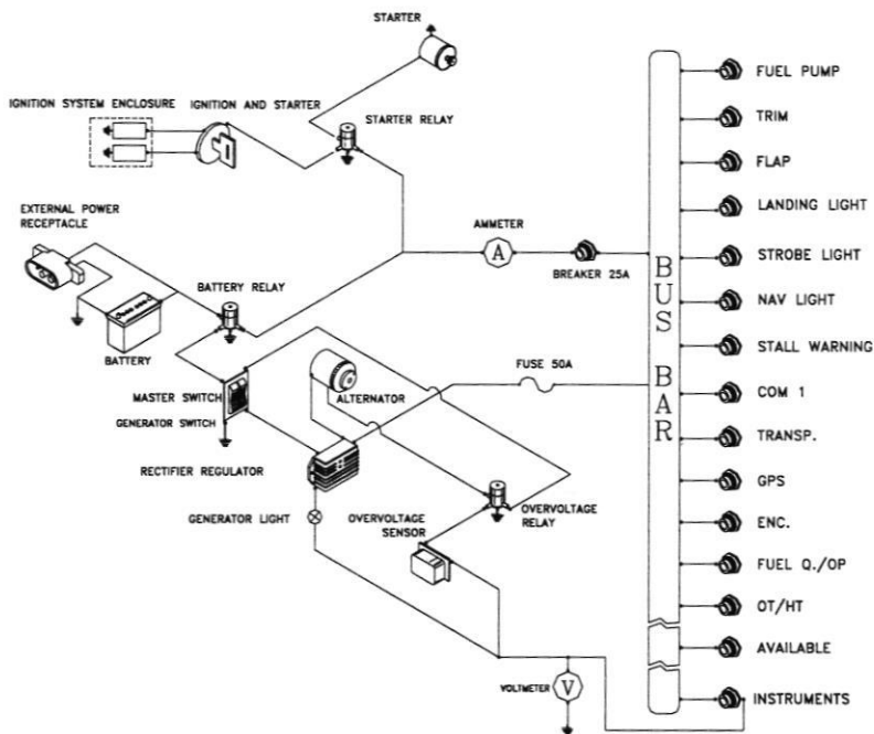
FIG. 7-4. ELECTRICAL SYSTEM SCHEMATIC
