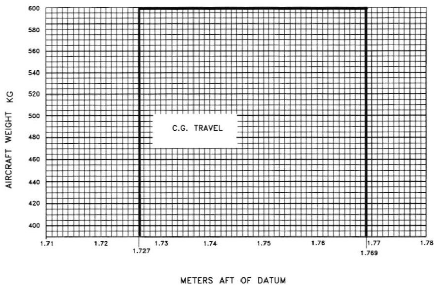
Fig 6-2. C.G. RANGE CHART.
